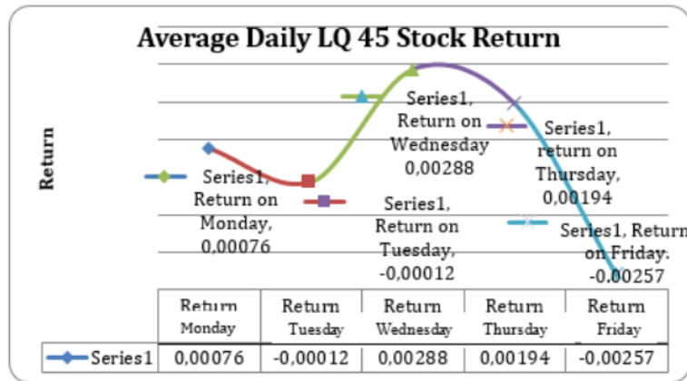
Figure 3. Average Daily LQ 45 Stock Return Chart
