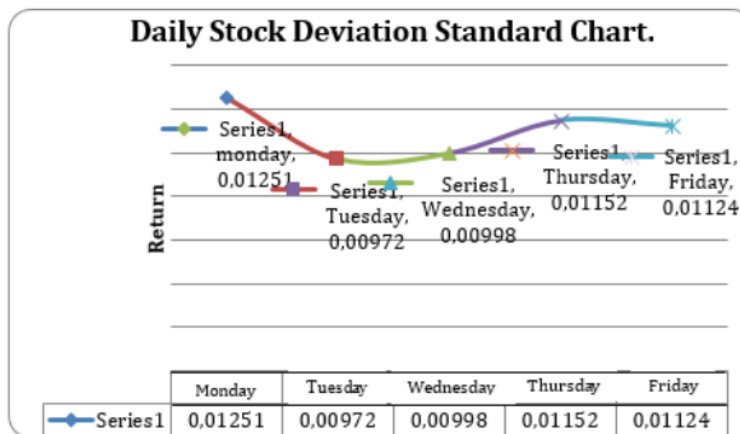
Figure 4. LQ 45 Daily stock Deviation Standard Chart
