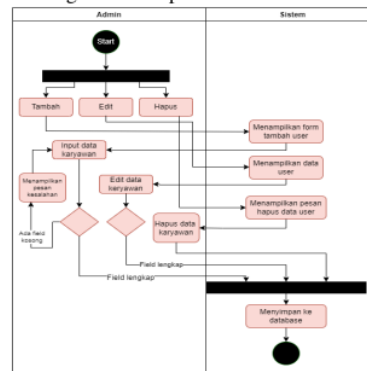
Gambar 5. Activity Diagram Kelola Data Karyawan
