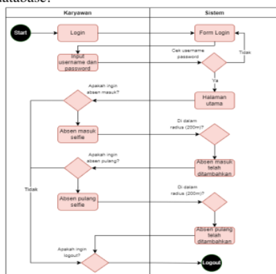
Gambar 6. Activity Diagram Absen Karyawan
