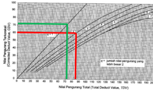
Grafik 3. Hubungan total deduct value dan correct deduct value STA 0+000 s/d 0+200
