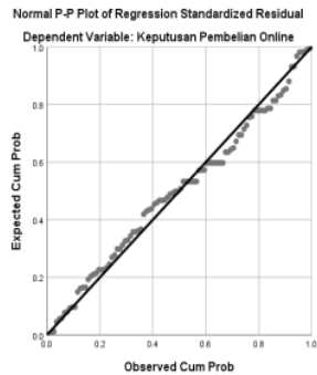
Gambar 2 Hasil Uji Normalitas Grafik Probability Plot
