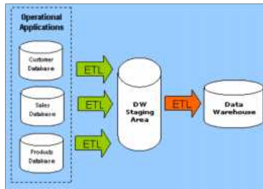
Gambar 1: Staging Area
