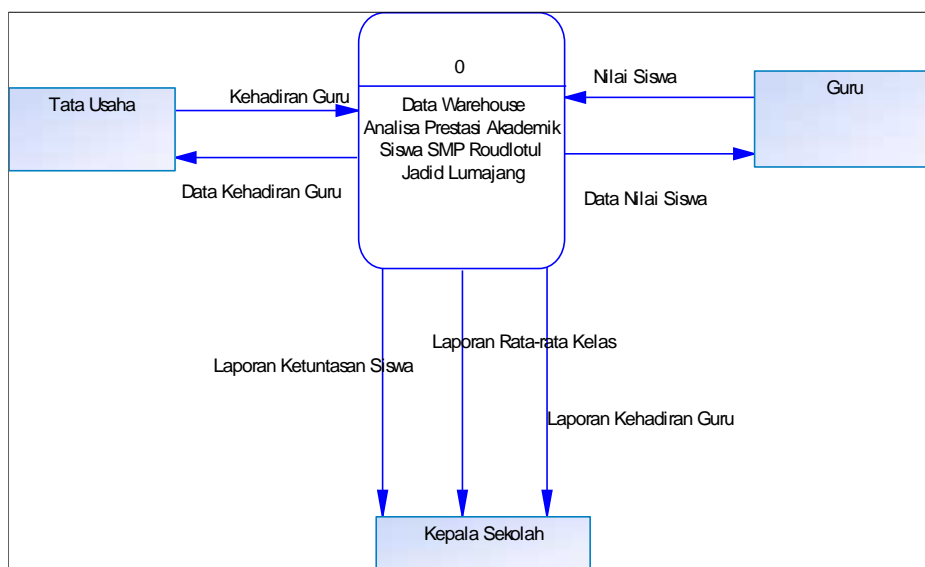
Gambar 7: Context Diagram
