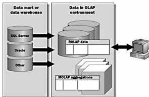
Gambar 5: HOLAP
