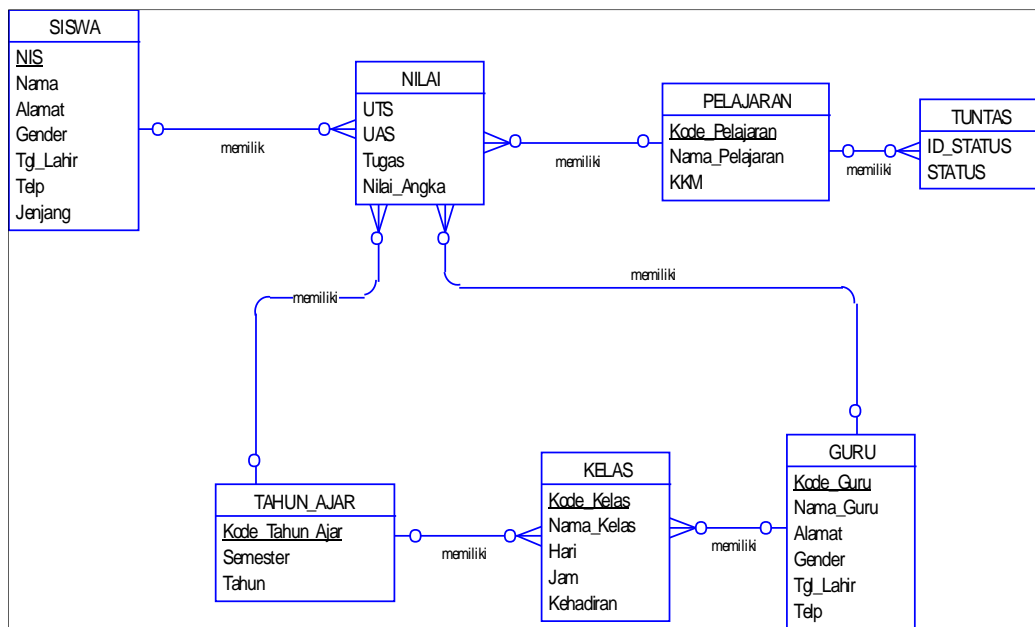
Gambar 9: CDM
