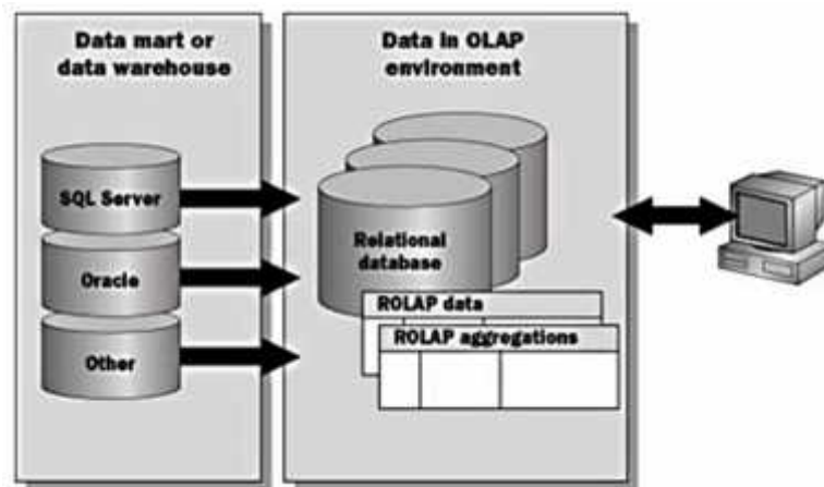
Gambar 4: ROLAP
