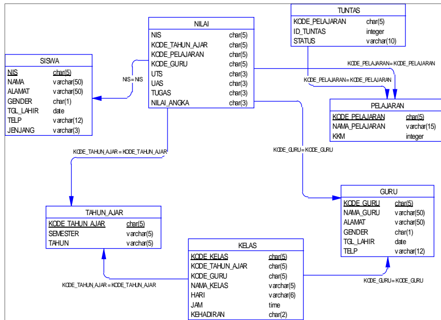
Gambar 10: PDM
