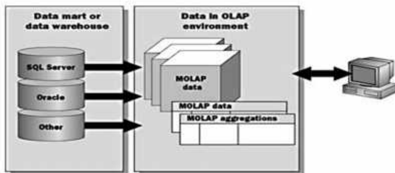
Gambar 3: MOLAP
