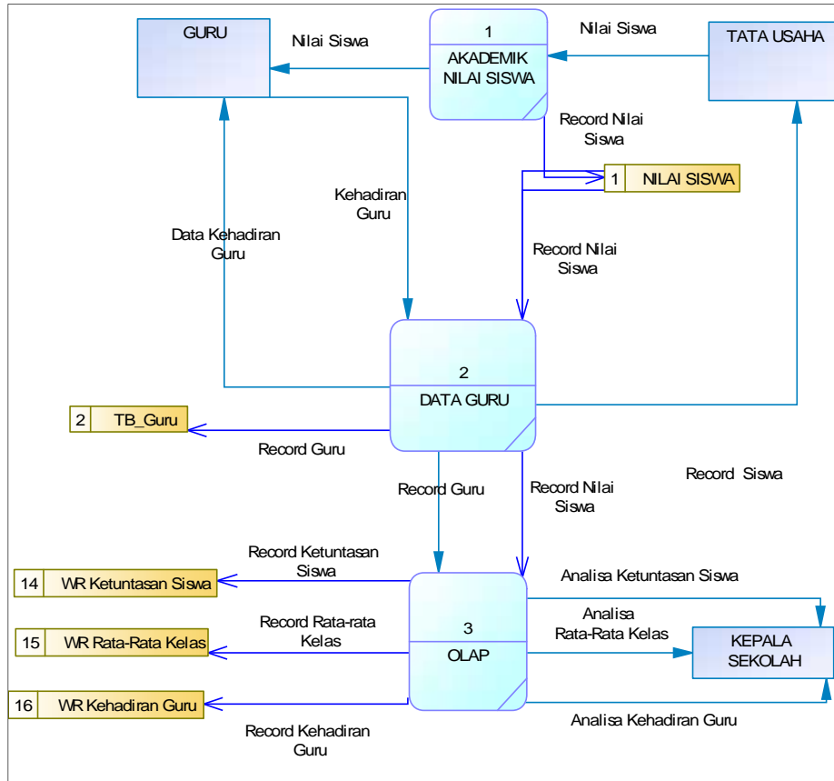
Gambar 8: DFD Level 1
